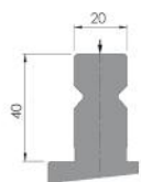
NS I New Standard I adaption
